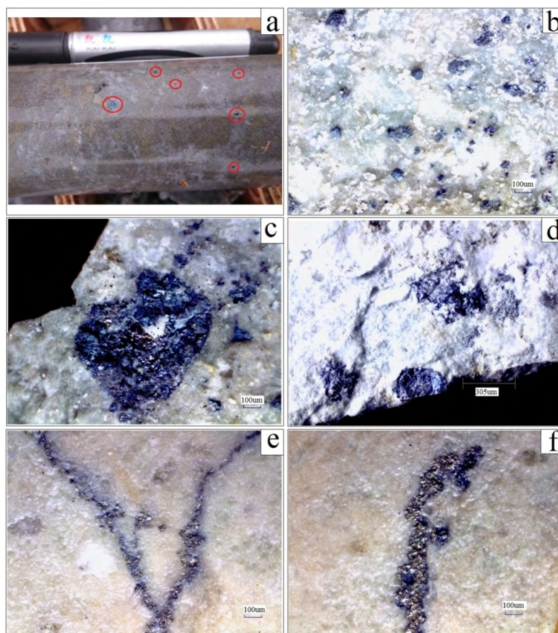
Fig. 7. Sulfide mineralization style of Reza gold deposit: a) covellite minerals grains into secondary quartzite (from core piece); b) covellite grains (little size); c) covellite-pyrite +/- wolframite (high grade by XRF-?) minerals grains (coarse size); d) covellite +/- wolframite (high grade by XRF-?); e) & f) covellite-pyrite veinlets in rhyodacite (?).
